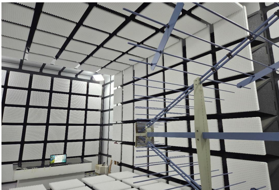
Radiated Susceptibility
